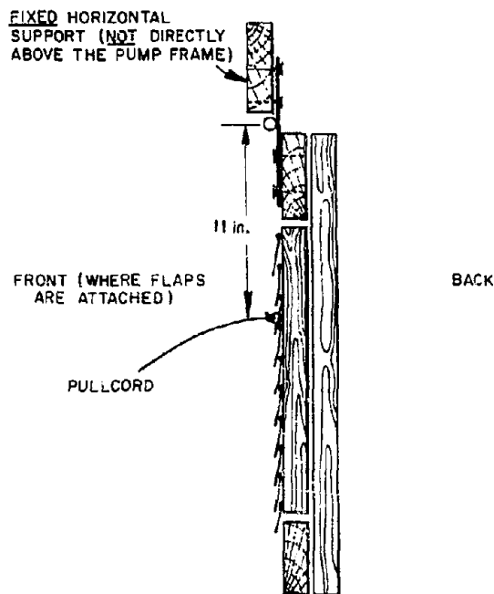
Fig. B-12. Side view of assembly.
